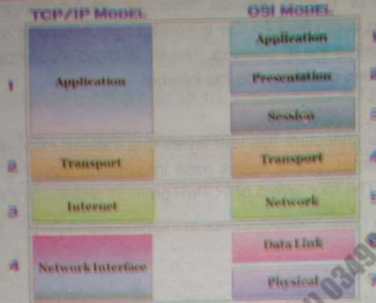
Fig.5.27 Comparison between TCP/IP and OSI Models
