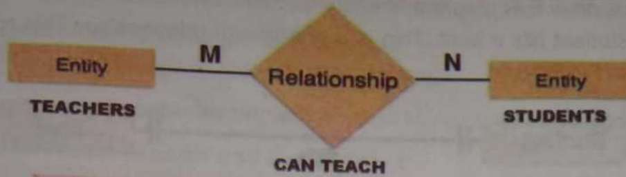
Fig.7.15 Many-to-many Relationship
