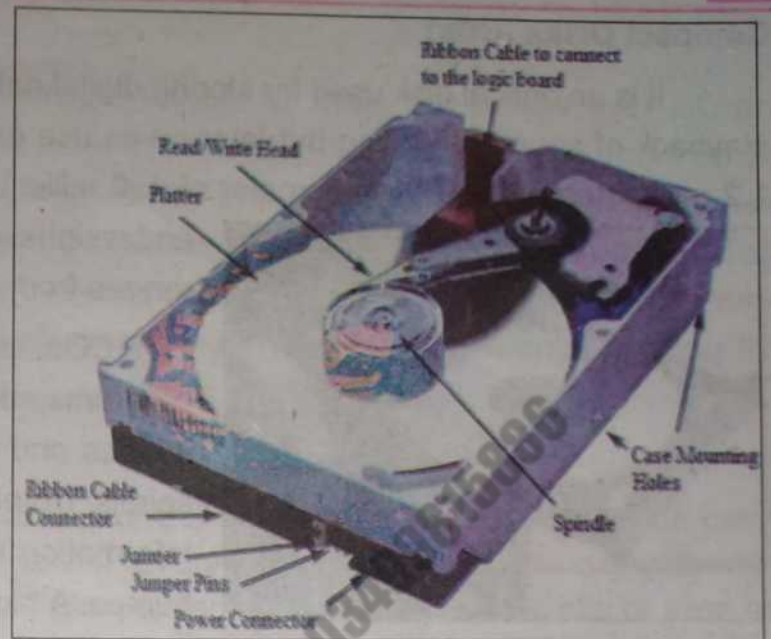
Fig.2.8 Hard Disk
